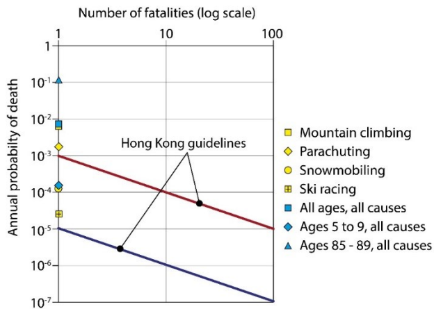
Figure 8. Accepted individual risks (Thomas and Hrudey 1997; Hutchinson2011 Personal comm..)
