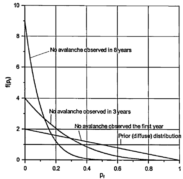
Figure 14. Probability distribution of annual avalanche probability 0, 1, 3 and 8 years of observations of no avalanche (Harbitz et al 2001).
