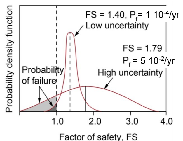
Figure 1 Factor of safety and probability of failure.
